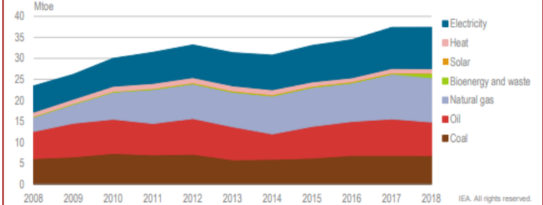
Figure 4.5 Energy consumption in industry by fuel, Turkey, 2008-18
